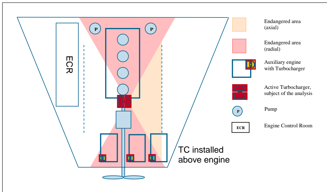
Figure 1: Conservative engine room arrangement for turbocharger application in 4-stroke Main Engine (single engine)
